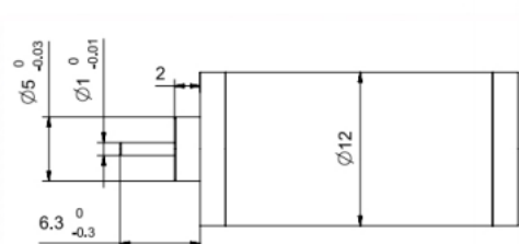
Motor Mounting Dimension Diagram :
