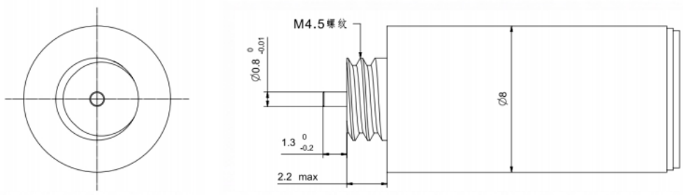
Motor Mounting Dimension Diagram :
