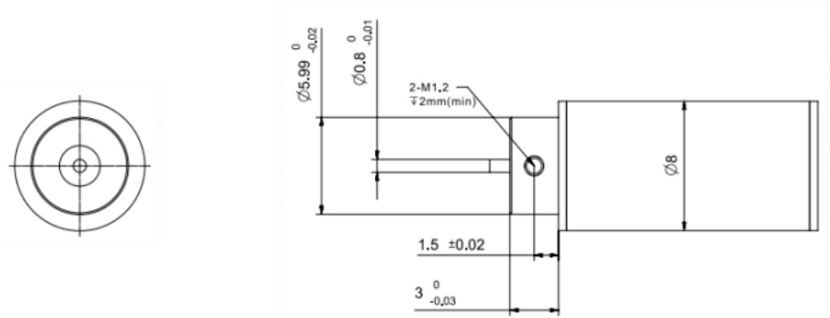
Motor Mounting Dimension Diagram :
