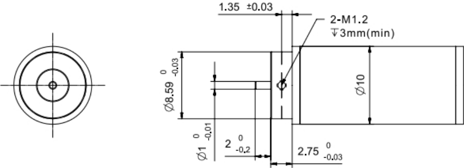
Motor Mounting Dimension Diagram :
