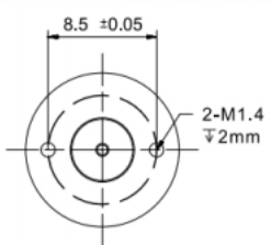
Motor Mounting Dimension Diagram :
