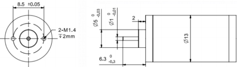
Motor Mounting Dimension Diagram :
